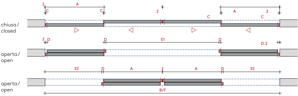
Binario due vie_4 divisori scorrevoli / Two ways rail_4 sliding partitions
