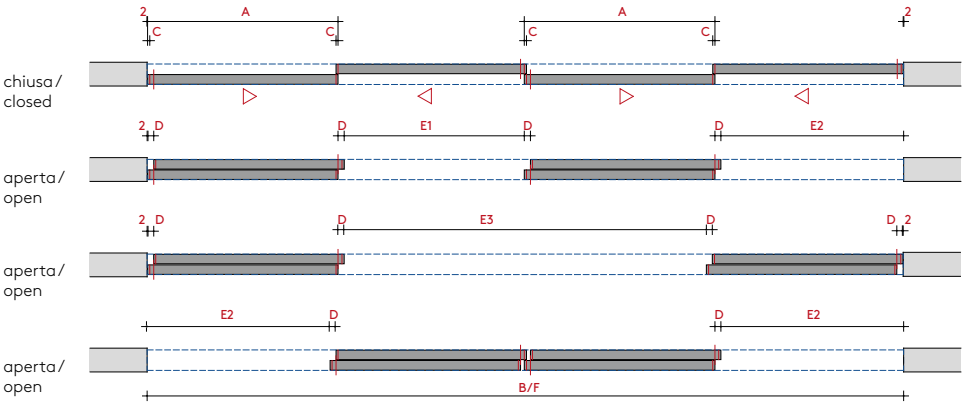
Binario due vie_4 divisori scorrevoli / Two ways rail_4 sliding partitions
